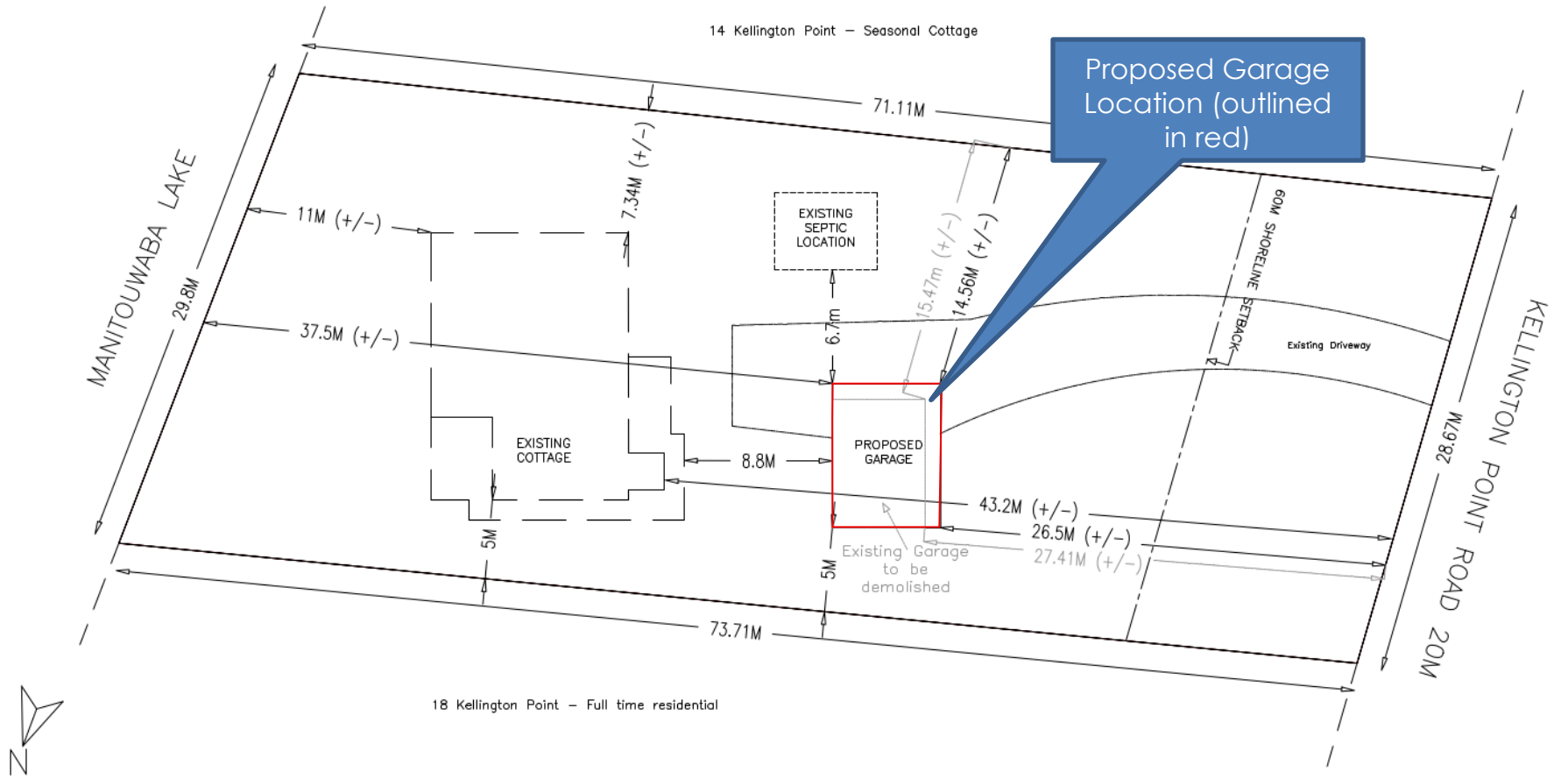
Figure 2: Proposed Site Plan (Excerpt)
